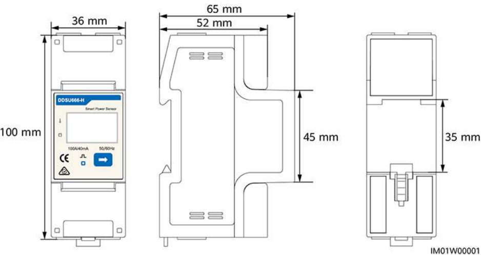
Figure 2-7 Product dimensions
