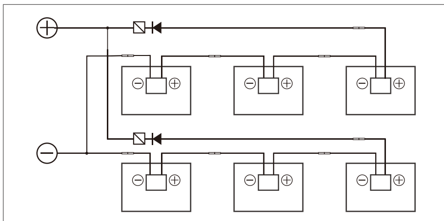
(Figure 9: Series-parallel connection diagram)
