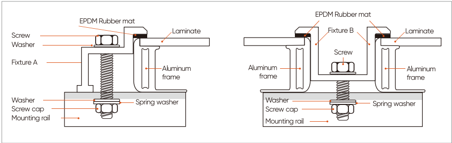
(Figure 5: Full-Screen PV Module Fixture Installation Diagram)
