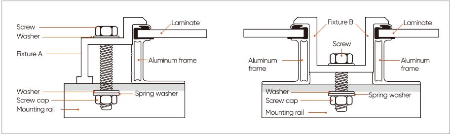
(Figure 4: Regular PV Module Fixture Installation Diagram)
