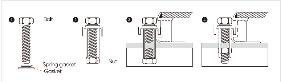
(Figure 6 Installation Detail with Side Fixture)
