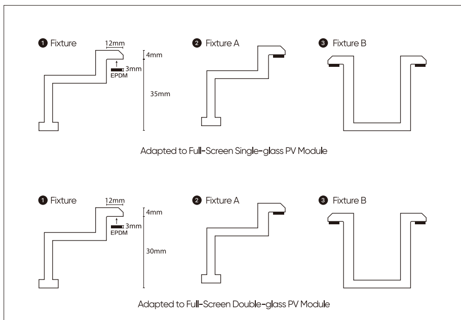
(Figure 3: Fixture Diagram of Full-Screen PV Module)
