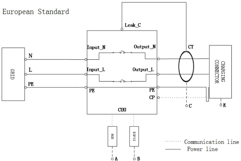
figure 3-1 Circuit diagram(European)
