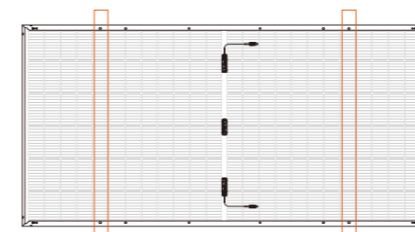
The outer four-hole bolt mounting, the beam perpendicular to the long frame
