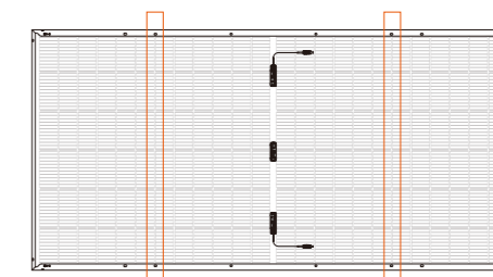
The inner four-hole bolt mounting, the beam perpendicular to the long frame
