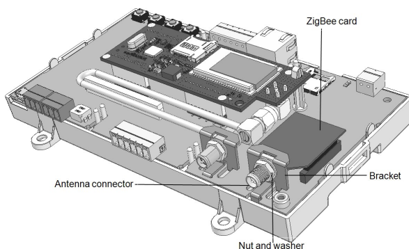
Figure 21: ZigBee Plug-in on a Commercial Gateway board
