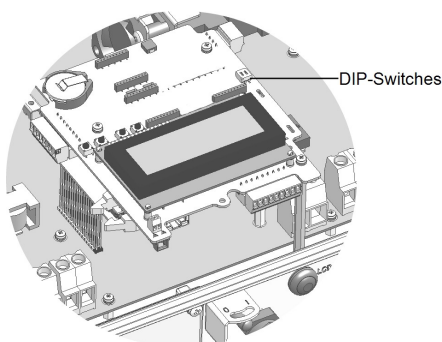
Figure 10: RS485 termination switch
