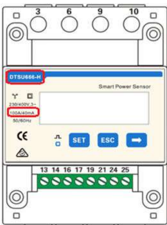
Figure 2-10 DTSU666-H
