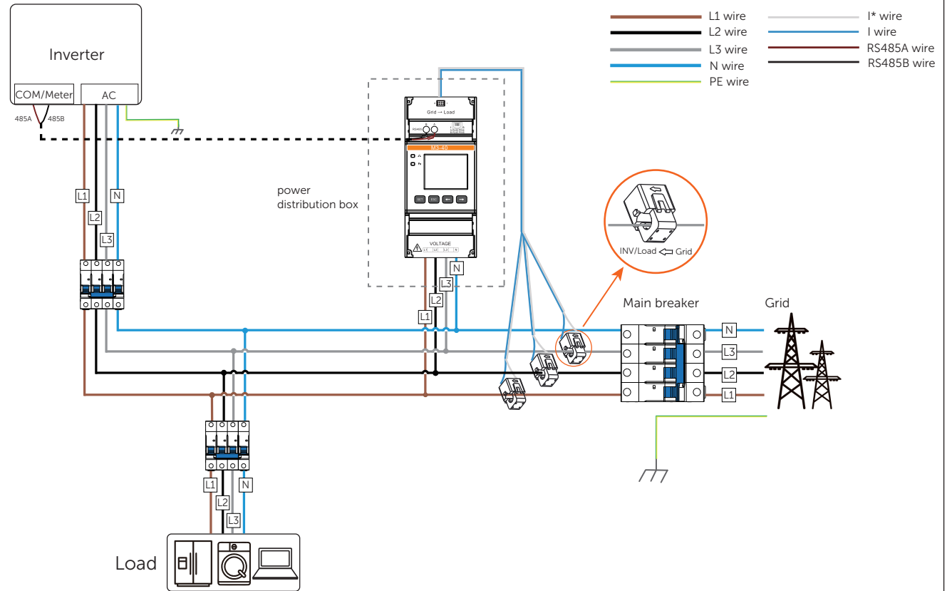
Figure 3-1 Networking through RS485 cable
