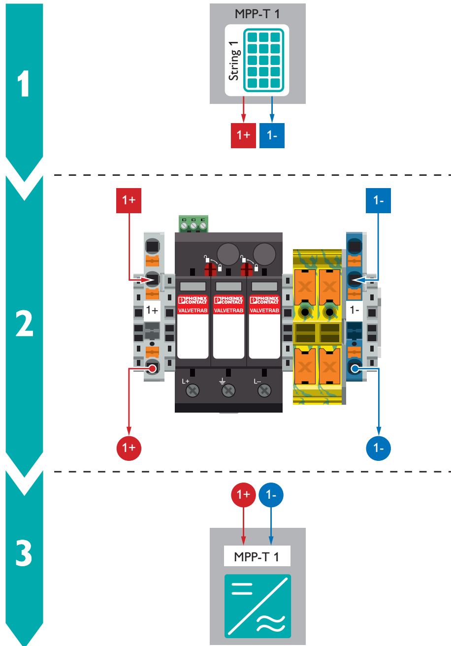
Connection diagram
